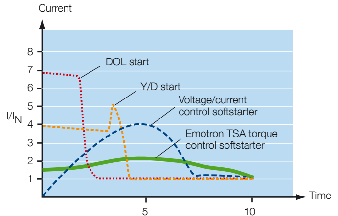
With an Emotron TSA the start current is up to 30% lower than with a conventional softstarter.
